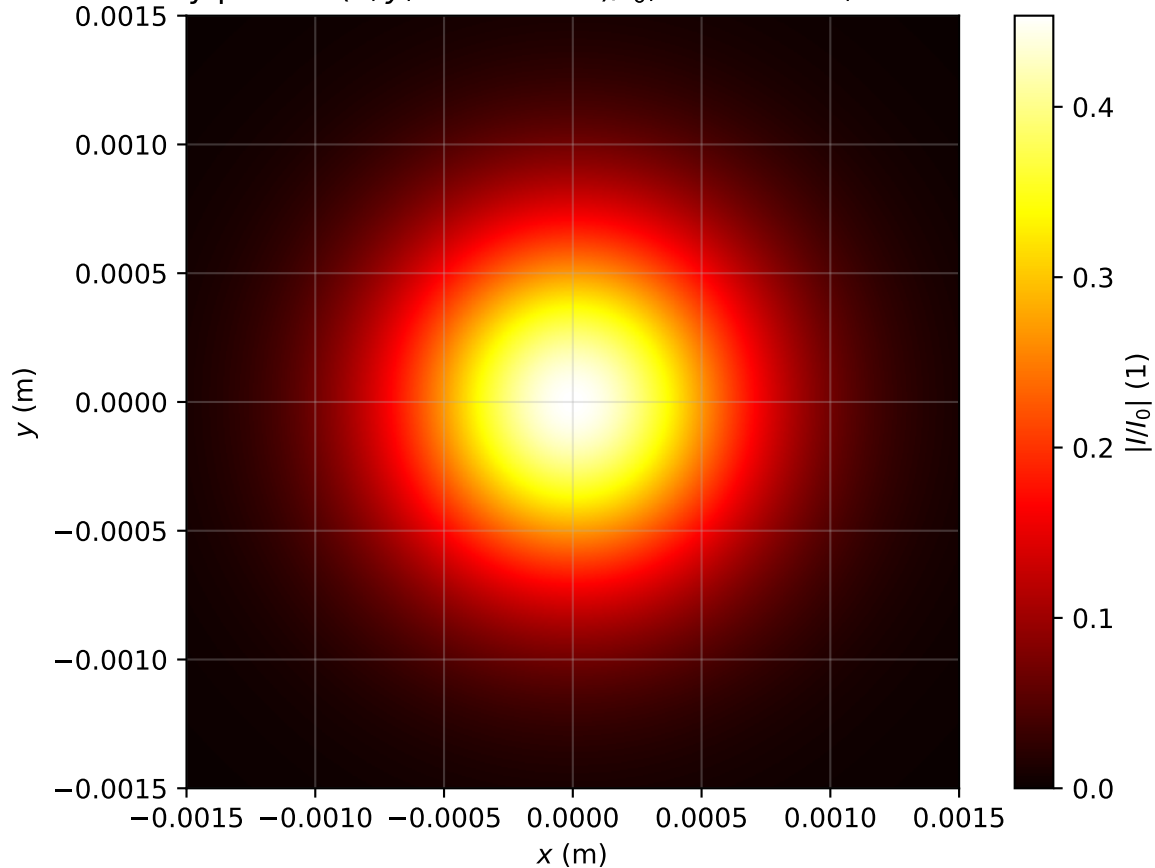
Intensity profile I(x, y, z = 3.582m)/I_0 , Pin=0.5Pcr, artificial time
